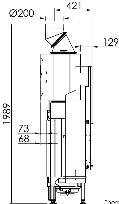
Thermobox, wide
