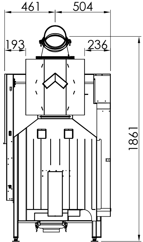
Thermobox, wide
