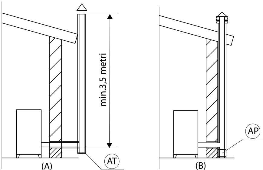
FIGURE 1 - FLUE
