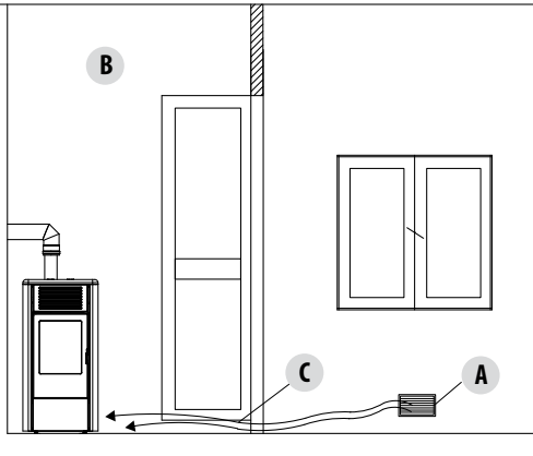
FIGURE 9 B - INDIRECTLY FROM THE ADJACENT ROOM
